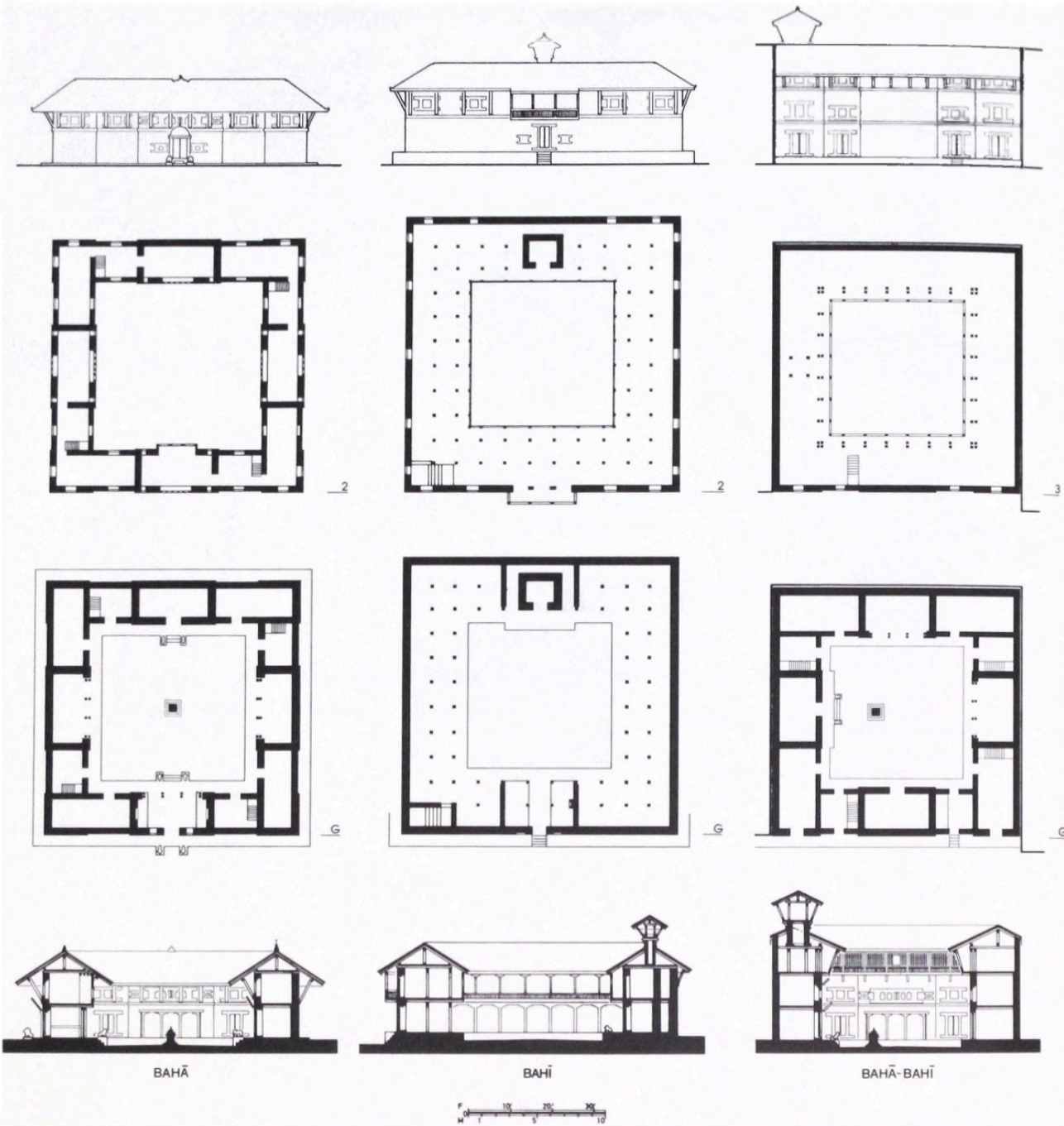
FIGURE 11. Comparison of three types of monastery quadrangle, a) bahā , b) bahī , and c) bahā-bahī : Chusya-bahal, Kathmandu, Duntu-bahil, and Nauddha-bahal, Patan; elevations, sections, and plans.
