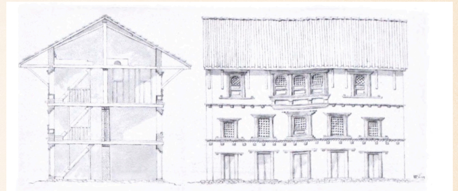
FIGURE 5. Elevation and section of a typical Newar farmhouse, showing construction and space allocation.
